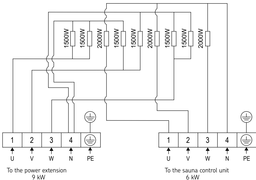
Figure 8. Wiring diagram CR150E
