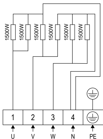
Figure 5. Wiring diagram CR90E
