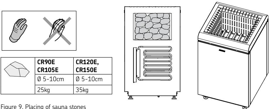
Figure 9. Placing of sauna stones
