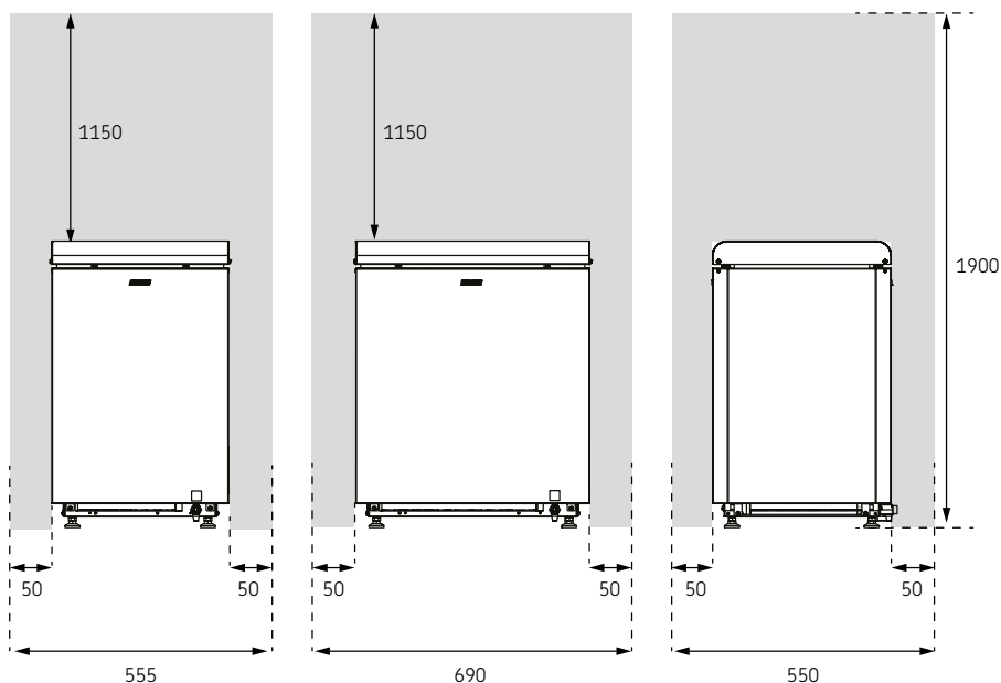
Figure 1. Safety distances
