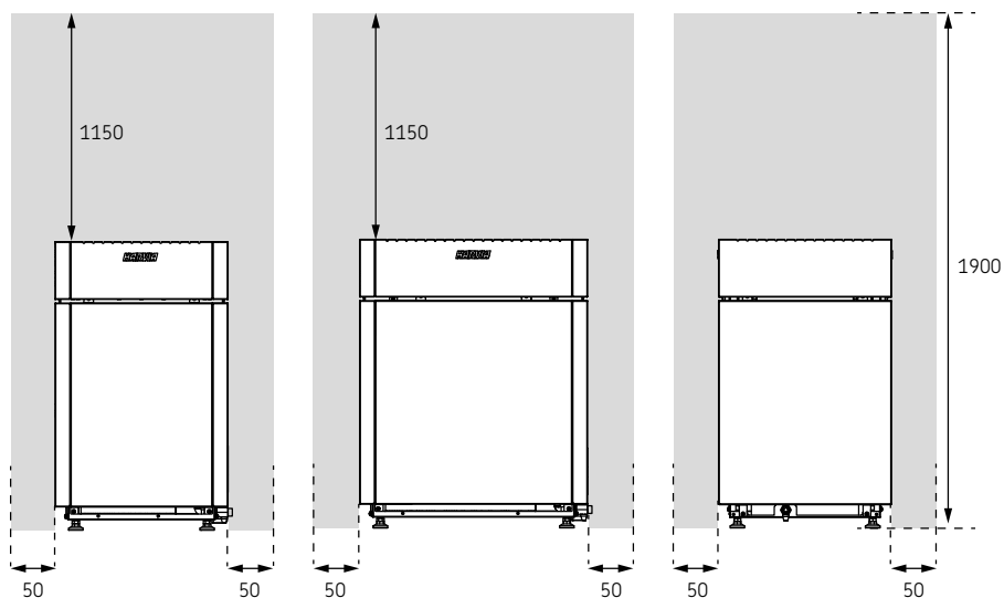
Figure 1. Safety distances
